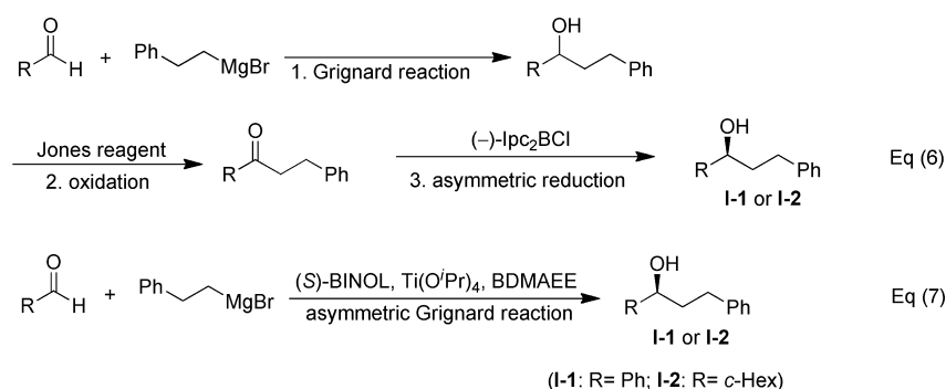
Scheme 3. Different Synthetic Methods of I-1 or I-2
